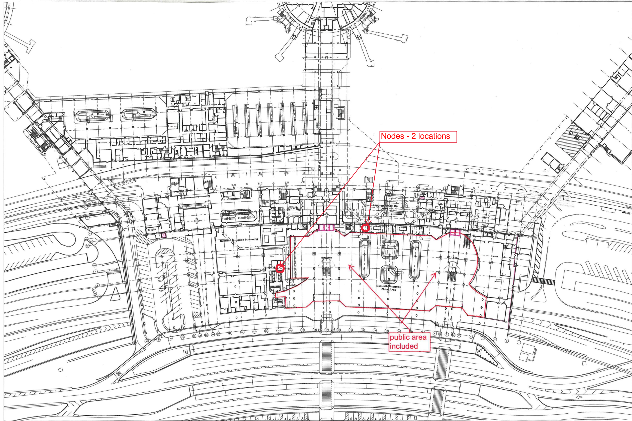
Level 1 Plan
