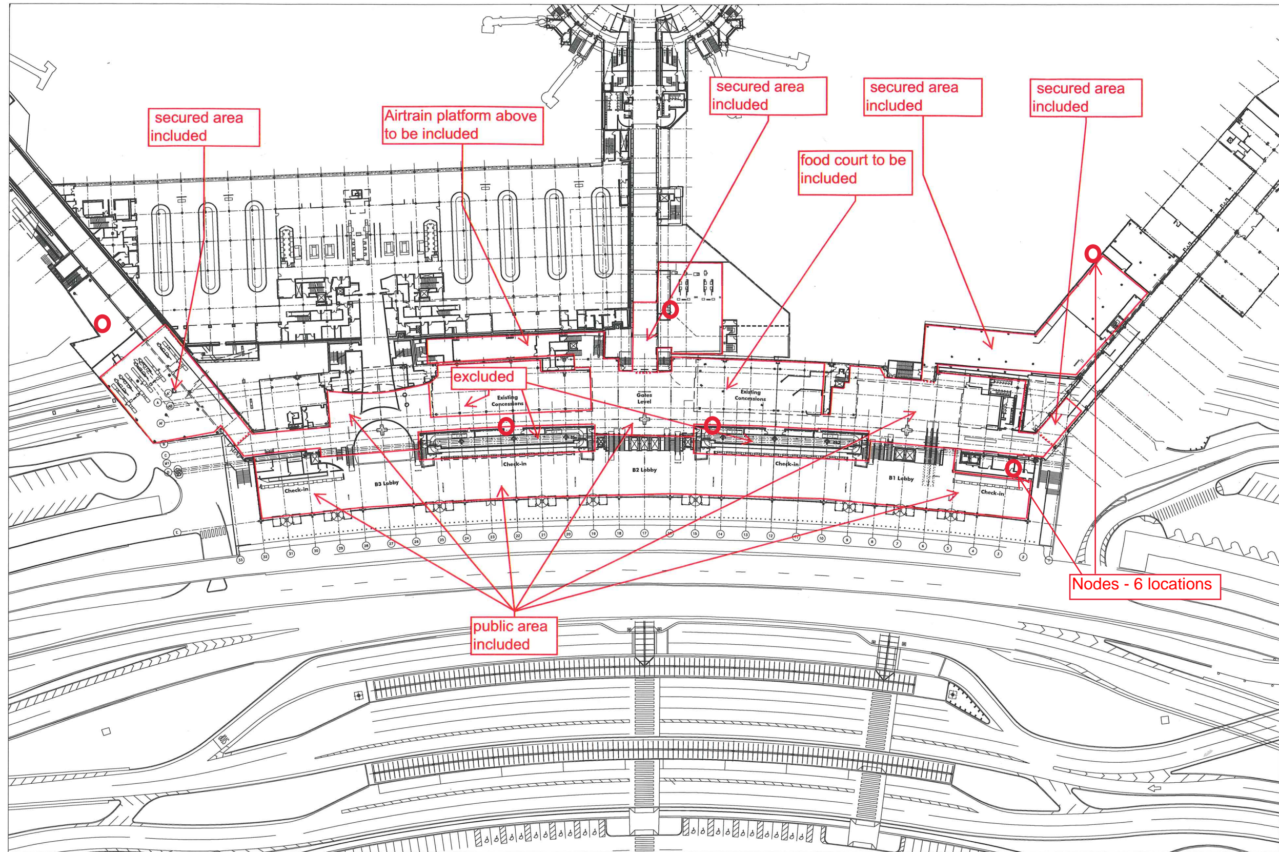
Level 3/Gates Level Plan
