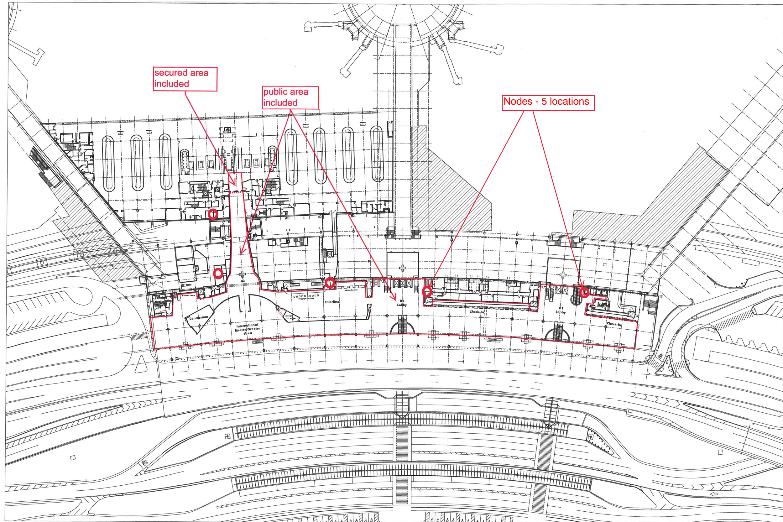
Level 2 Plan
