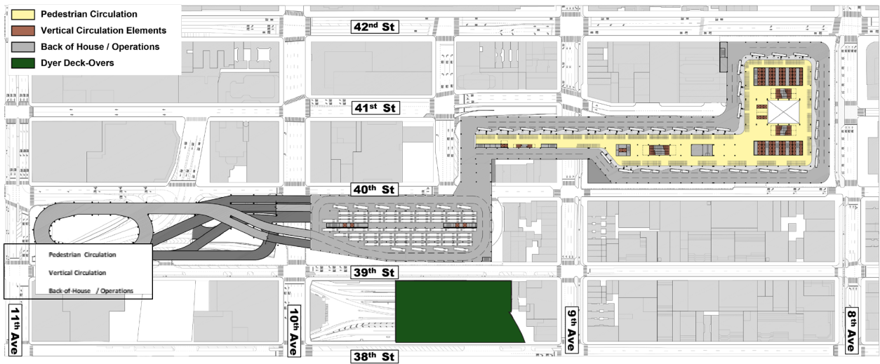
Figure B.4.1-11. Main Terminal Fifth and Sixth Level Floor Plan (Commuter, 40- to 45-foot, and 60-foot Buses)
