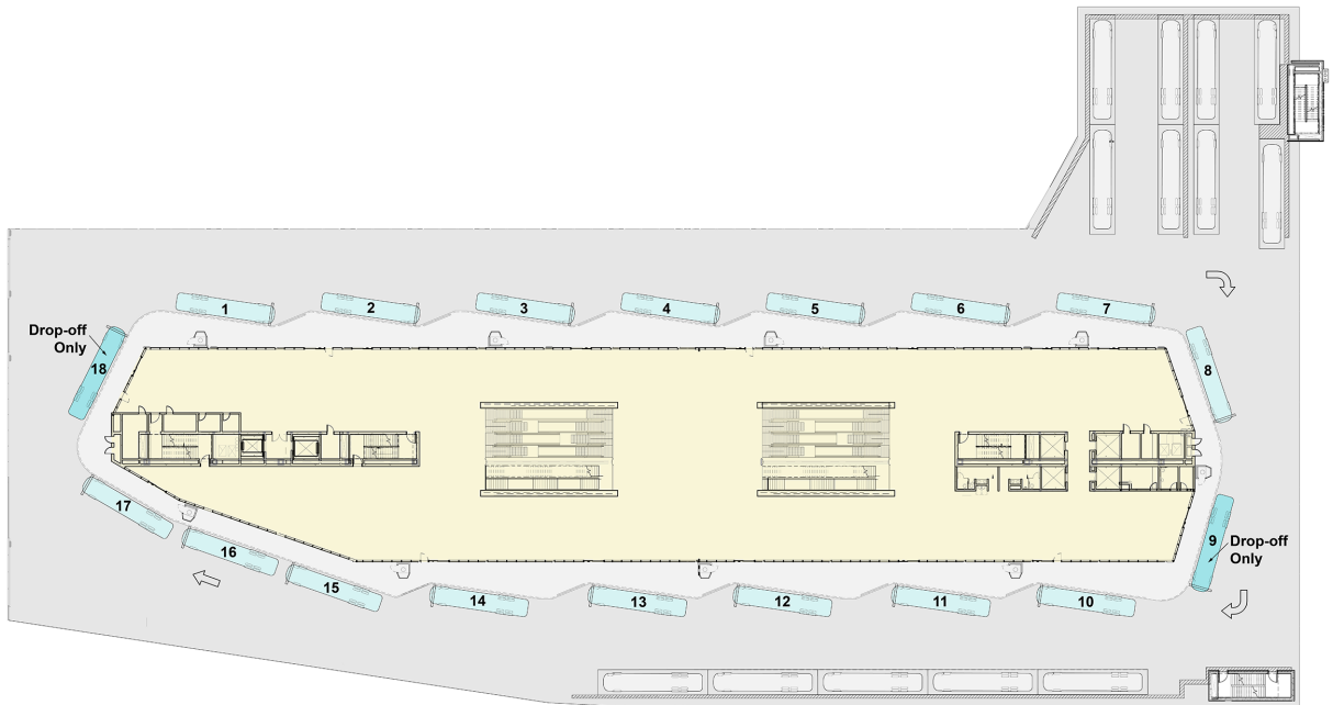
Figure B.4.1-6. SSF Temporary Operations Typical Floor Plan (Commuter, 40- to 45-foot Buses)
