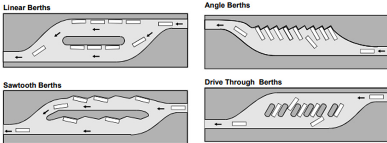
Figure B.4.1-2. Bus Gate Types Illustrated
