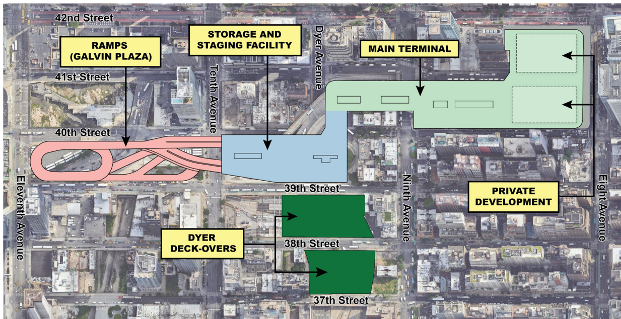
Figure B.4.1-1. Bus Terminal Replacement Project
