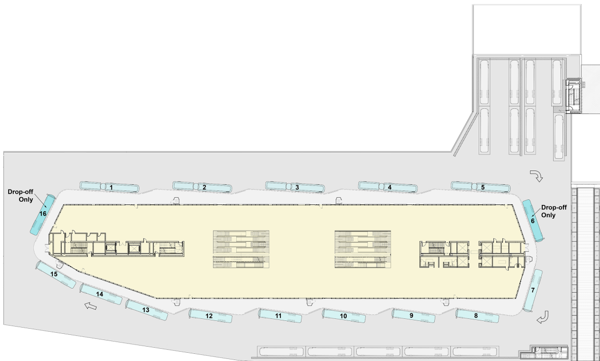
Figure B.4.1-7. SSF Temporary Operations Typical Floor Plan (Commuter, 40- to 45-foot, and 60-foot Buses)
