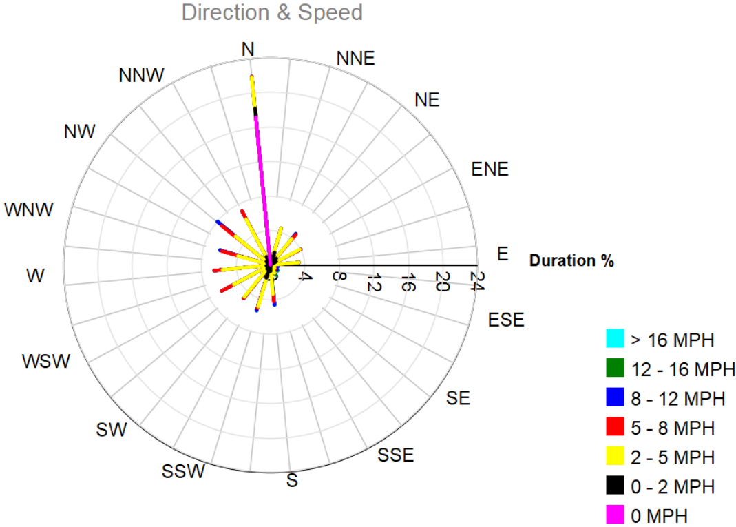
Wind Direction & Speed Relative Distribution
