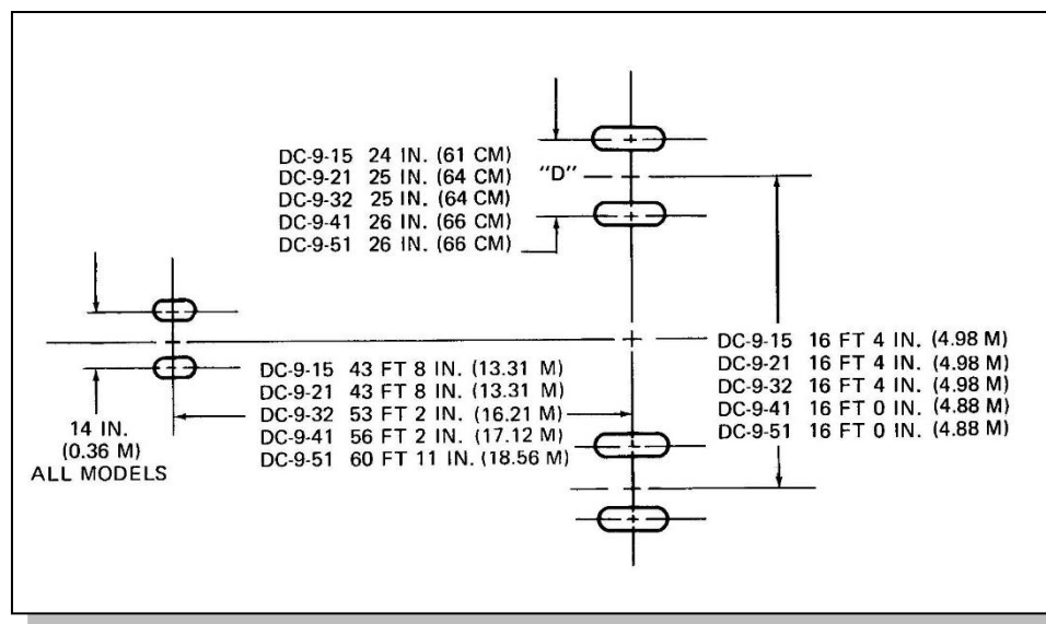
Figure 3-N TEB Aircraft Loads
