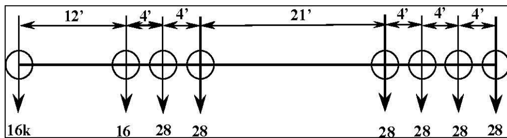
Figure 3-G NJDOT LRFD Permit Vehicle, (200 Kips)
