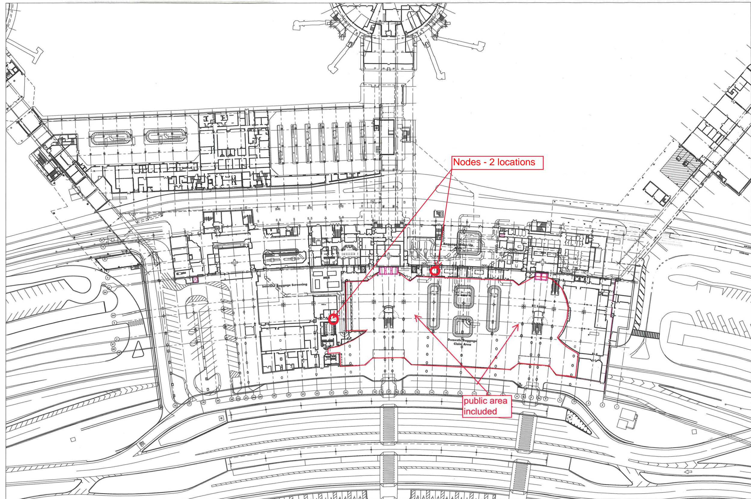
Level 1 Plan
